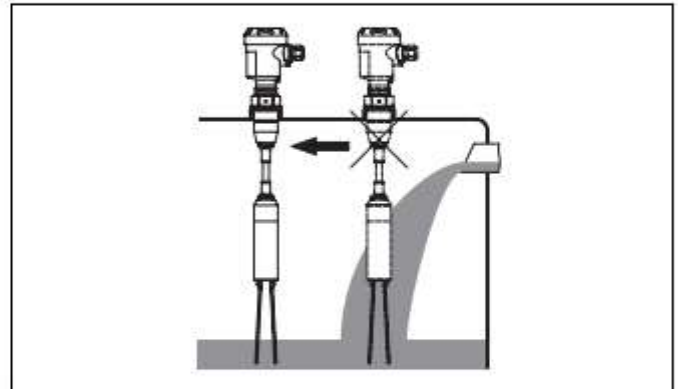
Fig. 4: Inflowing medium
