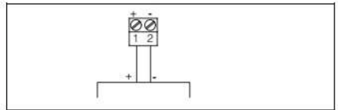
Fig. 15: Wiring plan, single chamber housing
