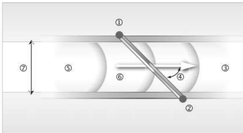
Figure 1-1: Measuring principle
