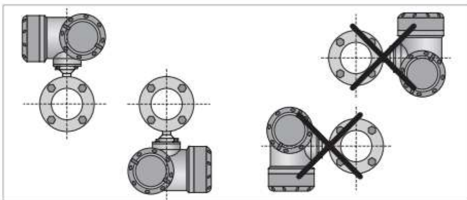
Figure 3-2: Mounting position
