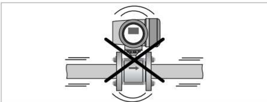
Figure 3-5: Avoid vibrations
