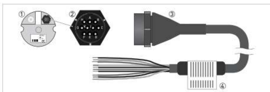
Figure 4-1: I/O cable
